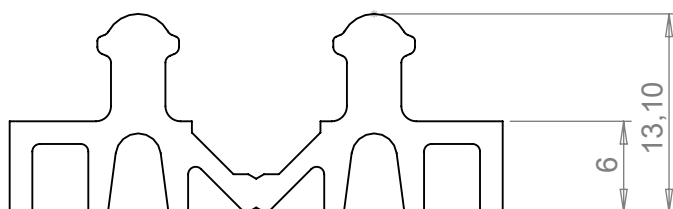
Rail Securitrack 60363N 401,66 g/m
